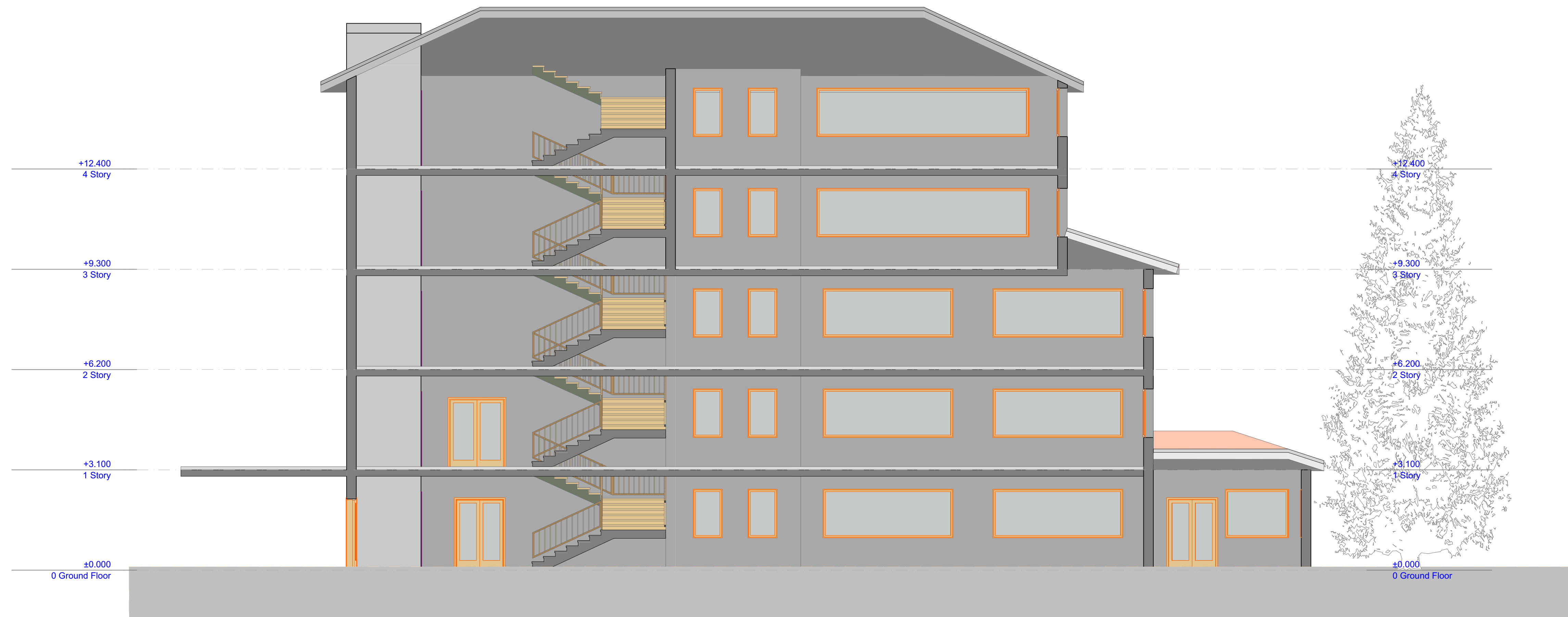
SECTION S-01
